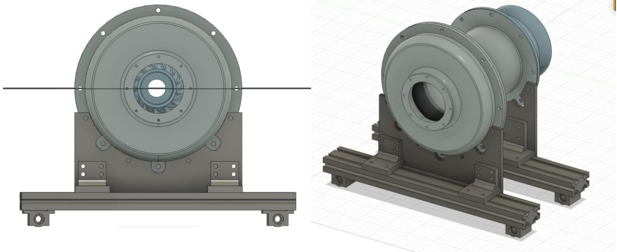
Designed and modeled thrust structure for Turbojet engine (~50 lb thrust capacity)
