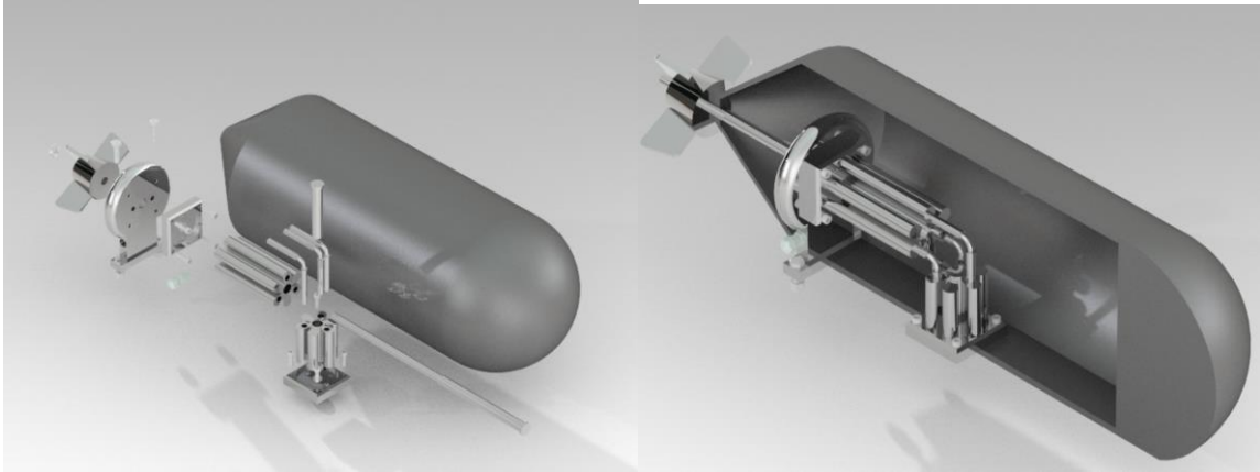
Designed and modeled functioning assembly of piston air engine with the uniquely designed base of a torpedo
